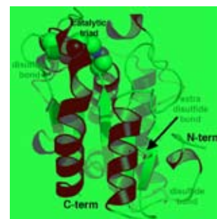
Figure 2. Crystal structure of A. oryzae cutinase (AoC) at 1.8Å resolution.
