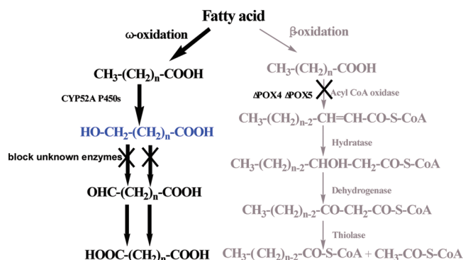
Figure 1. Two pathways for oxidation of fatty acids; the beta oxidation pathway can be blocked by deletion of both copies of the gene encoding the acyl CoA oxidase that catalyzes the first step in the pathway (POX4 and POX5). 21
