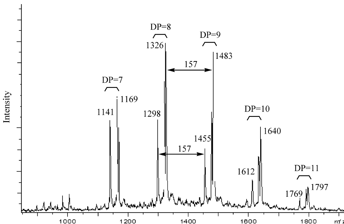
Figure 3. MALDI-TOF spectrum of oligo( \gamma -ethyl-L-glutamate) synthesized using 0.5 M L-glutamic acid diethyl ester hydrochloride, 8 mg/mL catalyst, at 40 °C for 20 min, pH 7.0, under noncontrolled pH conditions.
