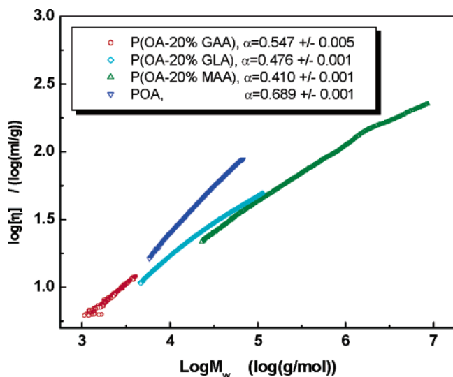
Figure 2. Intrinsic viscosity [\eta] as a function of the molar mass M for polyol containing polyesters and linear poly(octamethylene adipate) in THF solution at T = 25\text{ }^{\circ}\text{C} .
